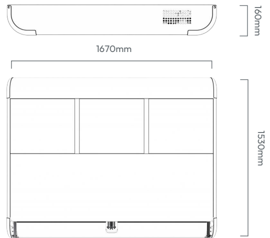
Dimensions (shrink)
